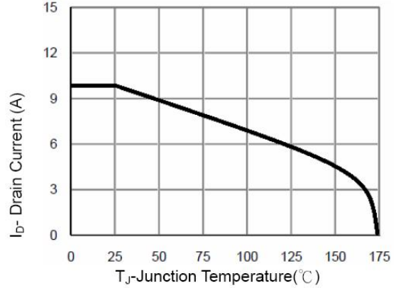
Figure 10 Current De-rating
