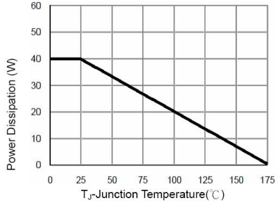
Figure 9 Power De-rating
