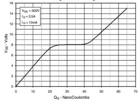
Fig. 10. Gate Charge
