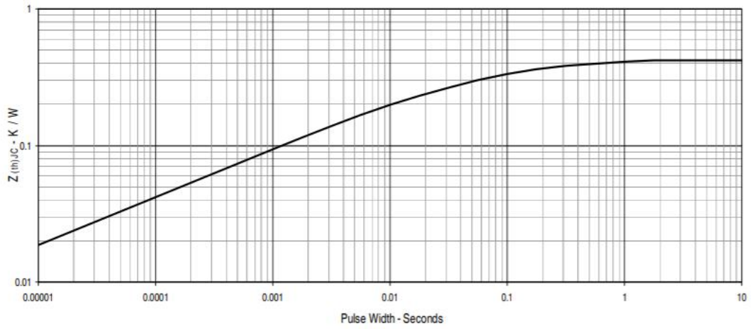
Fig. 13. Maximum Transient Thermal Impedance
