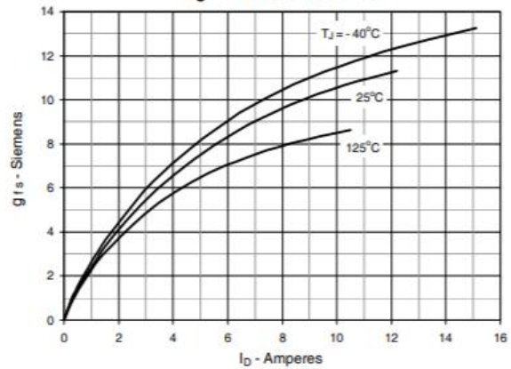
Fig. 8. Transconductance
