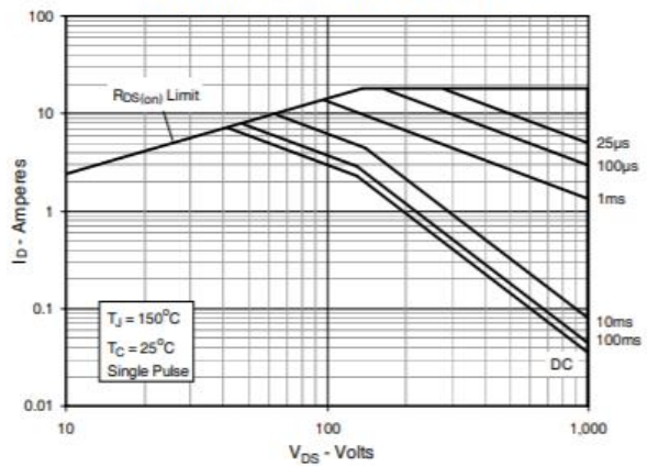
Fig. 14. Forward-Bias Safe Operating Area
