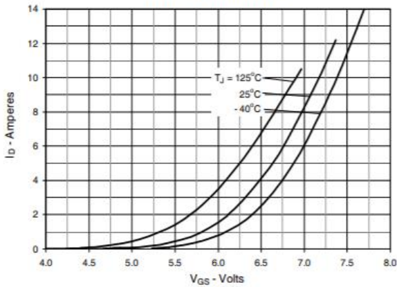
Fig. 7. Input Admittance
