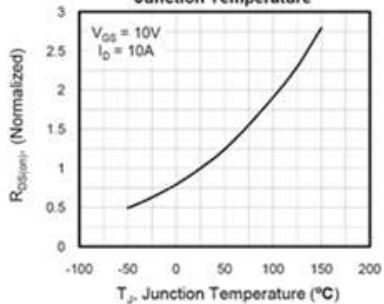
Figure 7. On-Resistance vs. Junction Temperature
