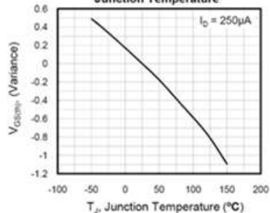
Figure 8. Threshold Voltage vs. Junction Temperature
