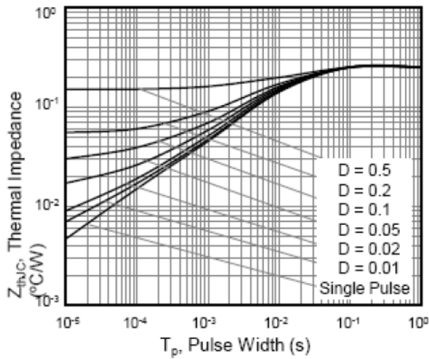
Figure 9. Transient Thermal Impedance for TO-247
