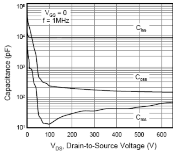
Figure 4. Capacitance
