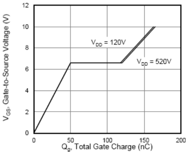
Figure 5. Gate Charge
