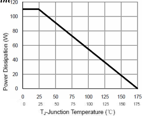
Figure 9 Power De-rating
