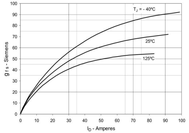
Fig. 8. Transconductance
