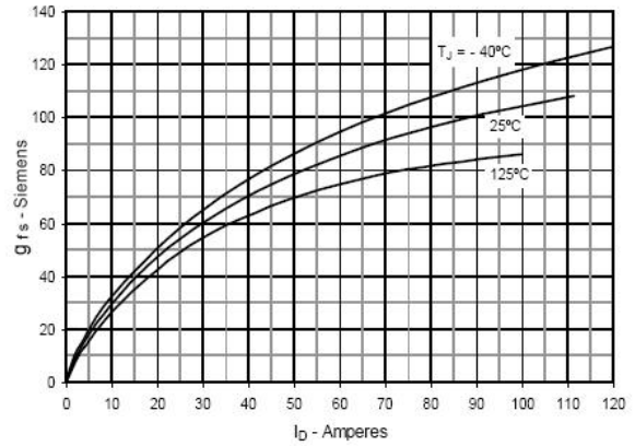
Fig. 8. Transconductance
