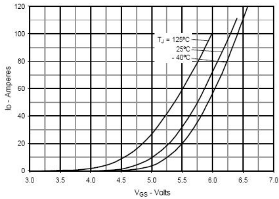
Fig. 7. Input Admittance
